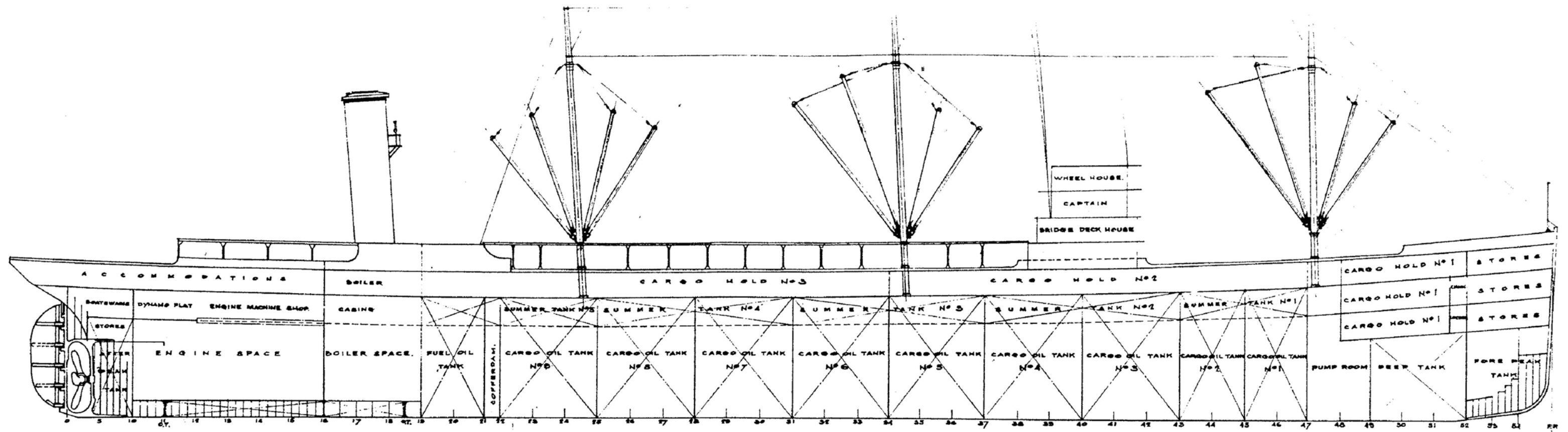
INBOARD PROFILE.
