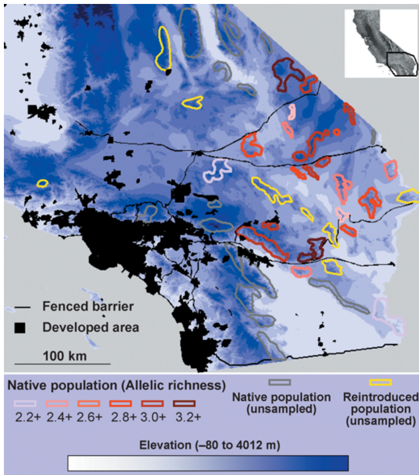
Fig. 1 Genetic diversity of 25 desert bighorn sheep populations in California, USA, with elevation and human-made barriers to dispersal (developed areas, fenced highways and canals). Unsourced populations were included when measuring isolation of sampled populations; sampling was not conducted in these locations because they were in military bases with restricted access, supported translocated sheep of known origin, or were outside the area defined for this study. Clusters of genetically diverse populations in high-elevation habitat with good connectivity may serve as genetic refugia during extended droughts and as sources of genetic diversity during more favourable climatic conditions.
