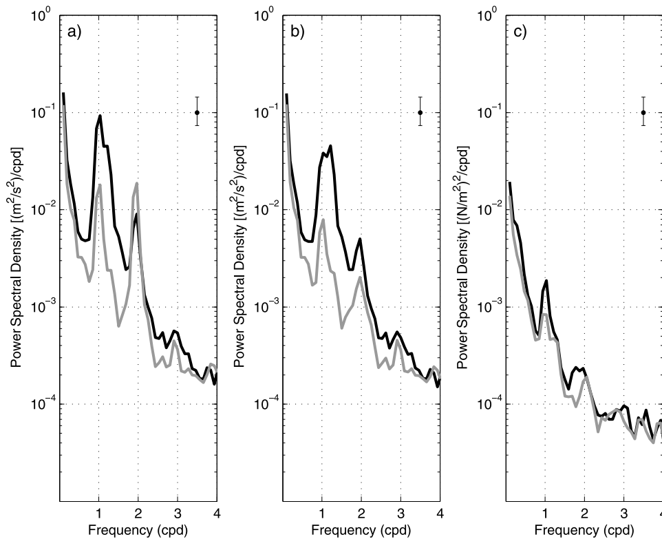
Figure 4. Power spectral densities of (a) HF radar current velocities, (b) residuals at location B, and (c) wind stress from buoy 46026 wind data for the year 1 September 2006 to 31 August 2007. The black line indicates clockwise rotation and the gray line indicates counterclockwise rotation. The 95% confidence interval is shown in the upper right corner. Frequency is in cycles per day (cpd).
