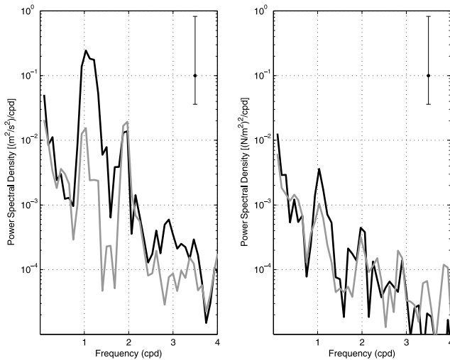
Figure 5. Power spectral densities of (left) HF radar velocities at location B and (right) wind stress from buoy 46026 wind data for the time period 1–26 September 2006. The black line indicates clockwise rotation and the gray line indicates counterclockwise rotation. The 95% confidence interval is shown in the upper right corner. Frequency is in cpd.
