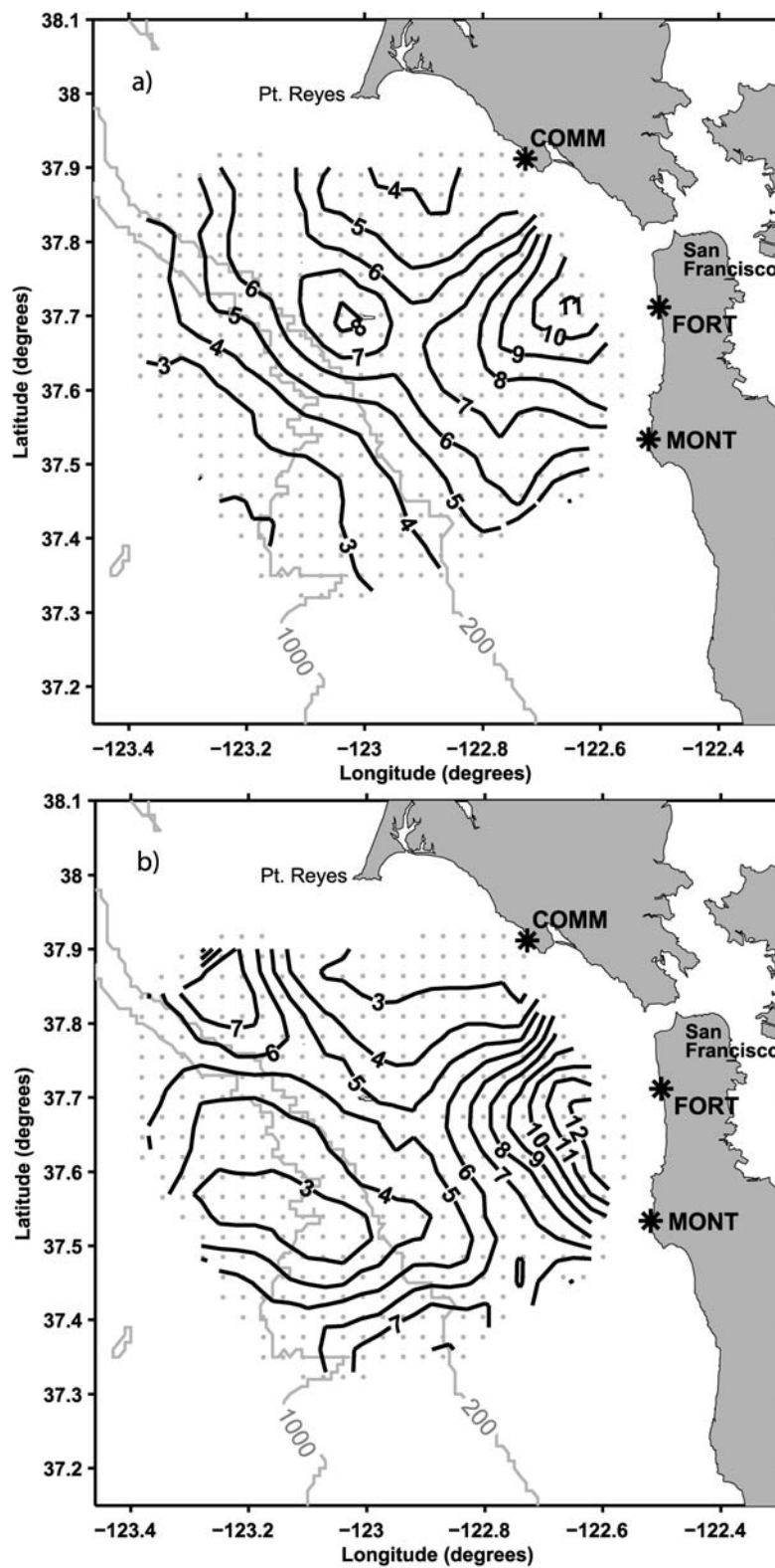
Figure 10. (a) K_1 and (b) M_2 tidal ellipse major axis amplitude contours in cm/s for the year September–August 2006–2007. Grey dots indicate HF radar data points.
