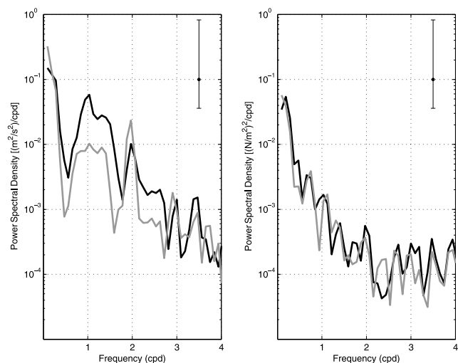
Figure 6. Power spectral densities of (left) HF radar velocities at location B and (right) wind stress from buoy 46026 wind data for the time period 15 February to 17 March 2007. The black line indicates clockwise rotation and the gray line indicates counterclockwise rotation. The 95% confidence interval is shown in the upper right corner. Frequency is in cpd.
