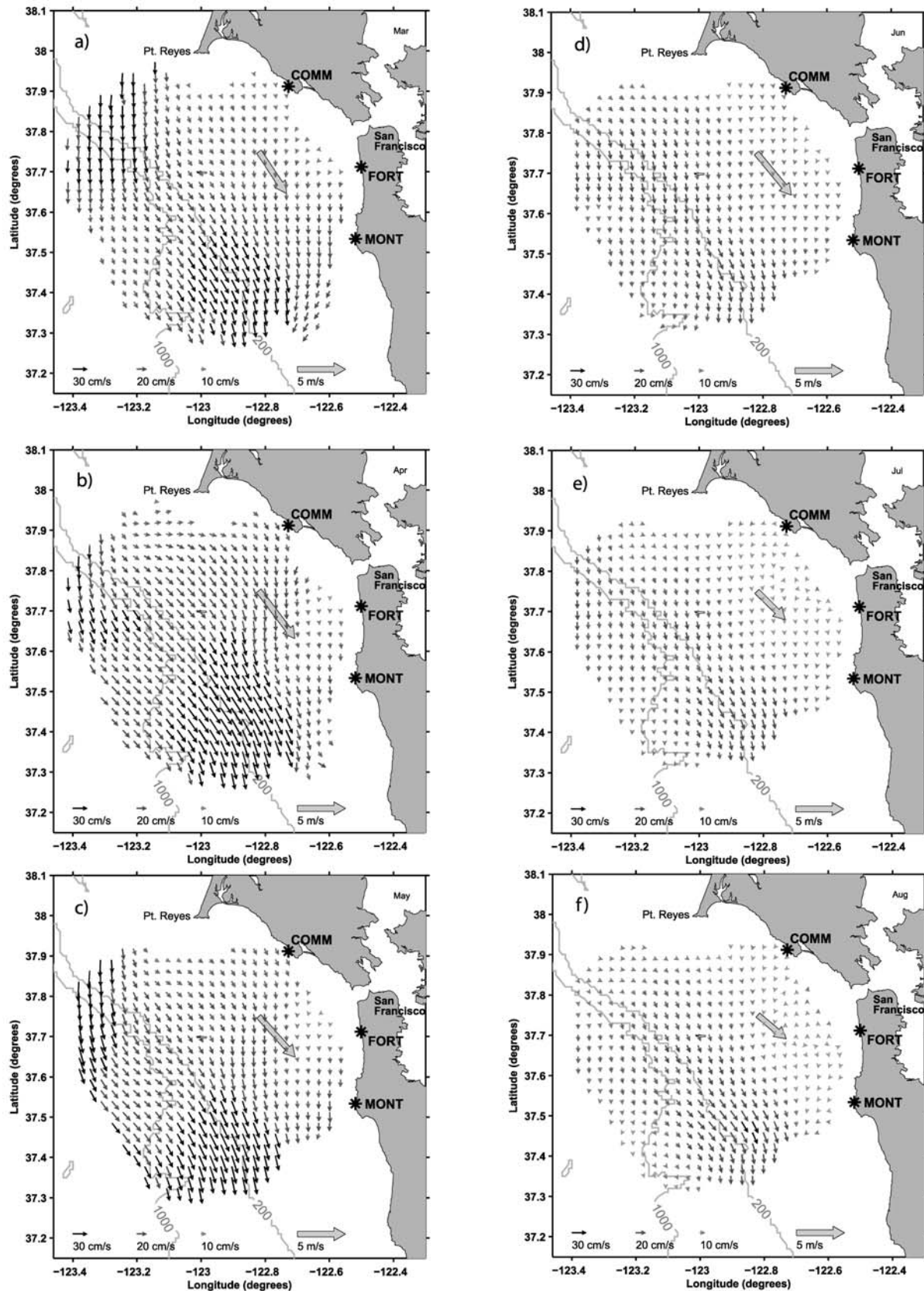
Figure 8. Mean monthly surface flow for (a) March, (b) April, (c) May, (d) June, (e) July, and (f) August. Magnitude is indicated by both the length and gray scale of the arrows. Black arrows indicate means greater than 25 cm/s. The large gray arrow indicates direction and magnitude of mean winds at buoy 46026 in m/s. Arrows are provided at the bottom for scaling.
