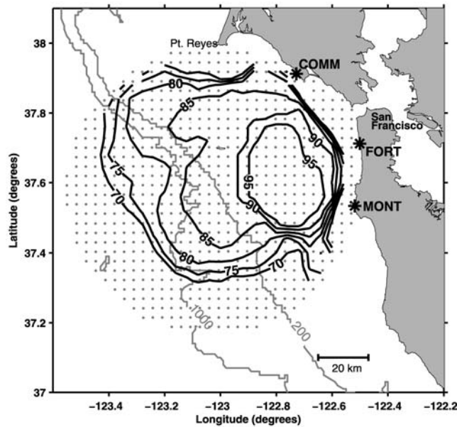
Figure 2. Percent contours of HF radar temporal data coverage for the year September–August 2006–2007. Grey dots indicate total vector data points on 3 km grid. Only data points with at least 70% coverage were used in this study. Contours below 70% are not shown.
