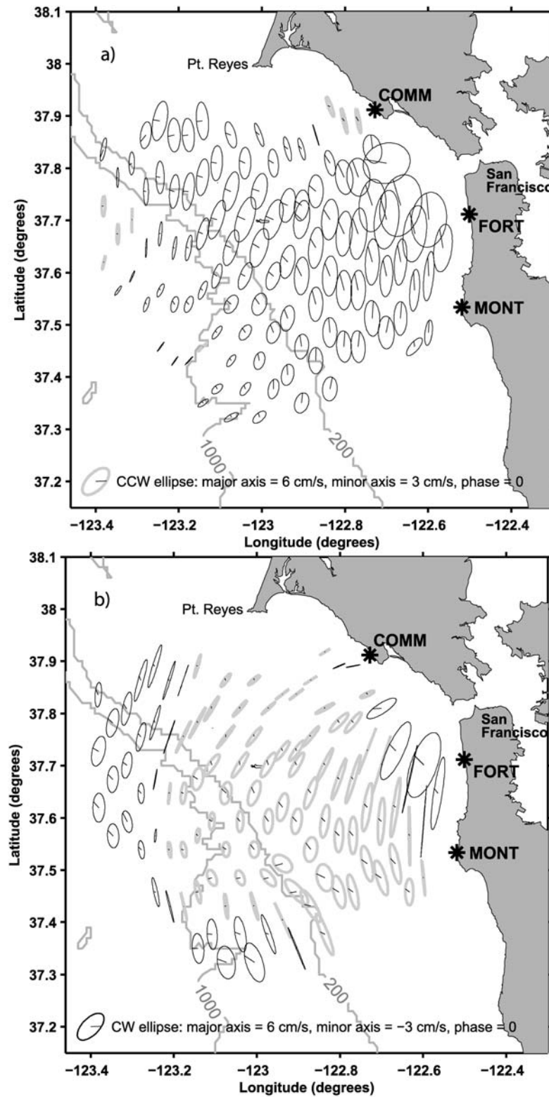
Figure 11. (a) K_1 and (b) M_2 tidal ellipses derived from the harmonic tidal analysis on a year of HF radar data (September–August 2006–2007). Ellipses are for every fourth HF radar data point. CCW ellipses are gray, CW ellipses are black, and black lines emanating from the center of ellipses denote phase relative to UT.
