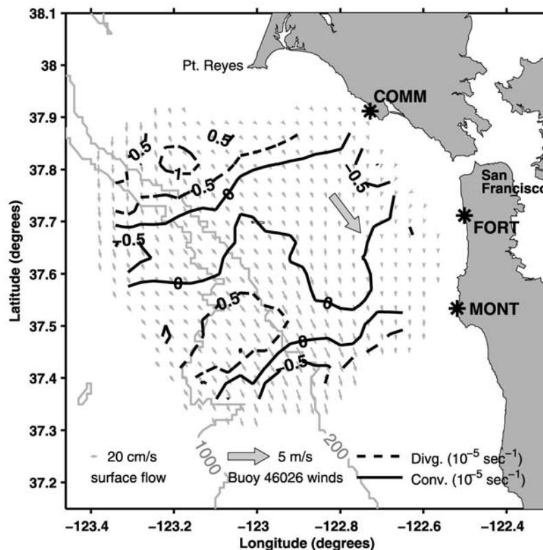
Figure 13. Mean divergence contours averaged over the beginning of the upwelling season of 2007 (March, April, and May). Dashed contours indicate divergence and solid contours indicate negative divergence (convergence) on the order of 10^{-5} \text{ s}^{-1} . Small gray arrows indicate mean surface flow scaled down to primarily show direction. The large gray arrow indicates magnitude and direction of mean winds at buoy 46026.
