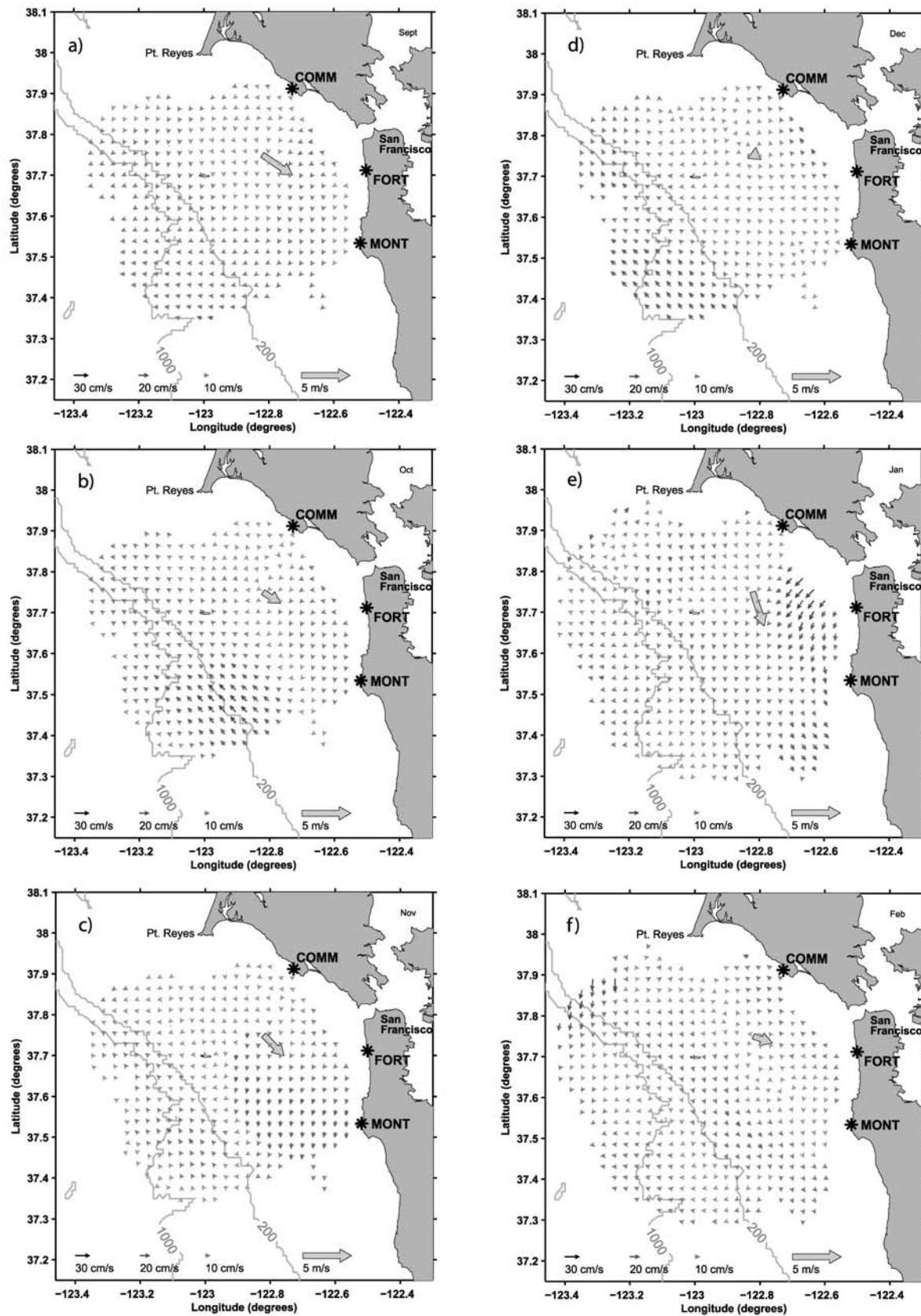
Figure 7. Mean monthly surface flow for (a) September, (b) October, (c) November, (d) December, (e) January, and (f) February. Magnitude is indicated by both the length and gray scale of the arrows. Black arrows indicate means greater than 25 cm/s. The large gray arrow indicates direction and magnitude of mean winds at buoy 46026 in m/s. Arrows are provided at the bottom for scaling.
