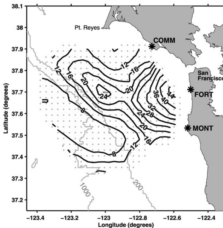
Figure 9. Percent total tidal variance contours for the year September–August 2006–2007. Grey dots indicate HF radar data points.
