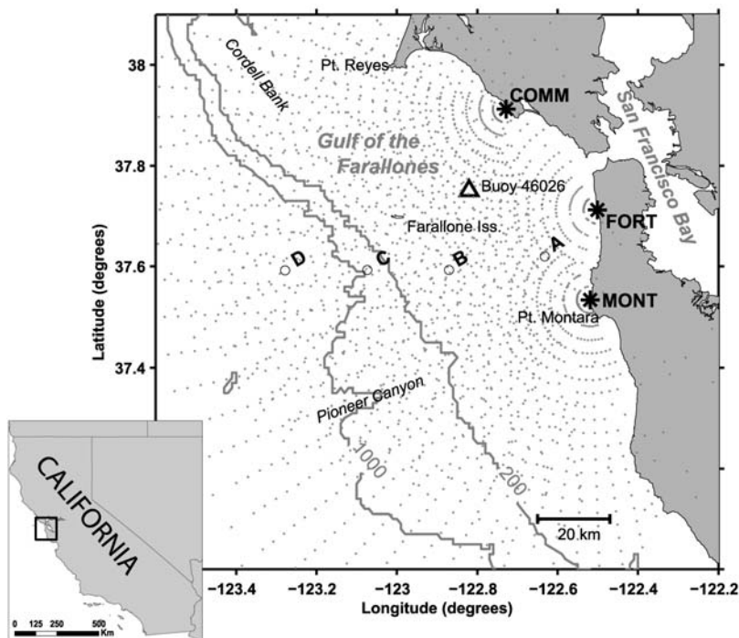
Figure 1. Gulf of the Farallones study area. The box in the index map of California outlines the study area. Grey lines denote the 200 and 1000 m bathymetry contours. CODAR stations are denoted with stars (COMM, Commonwealth; FORT, Fort Funston; MONT, Montara). Small gray points are radial data points for each station. Four cross-shore coordinate points used in detailed harmonic tidal analyses are labeled A ( 37.620^{\circ}\text{N} , 122.632^{\circ}\text{W} ), B ( 37.593^{\circ}\text{N} , 122.870^{\circ}\text{W} ), C ( 37.593^{\circ}\text{N} , 123.074^{\circ}\text{W} ), and D ( 37.592^{\circ}\text{N} , 123.278^{\circ}\text{W} ).
