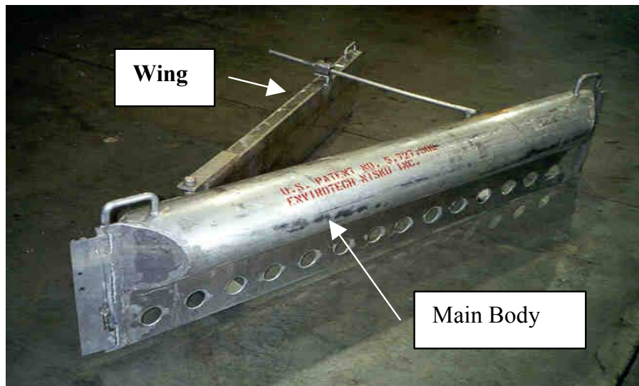
Figure 5-5. Boom deflector.
