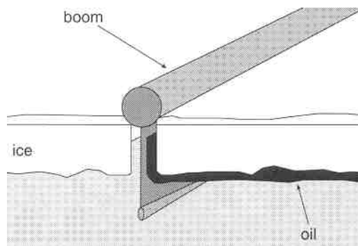
Figure 7-3. Boom deployed in ice slot.
