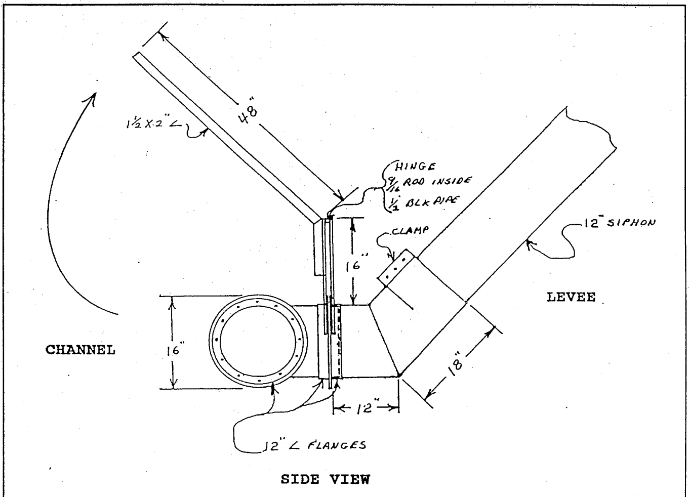
Figure 3 MODIFIED SWIVEL JOINT INSTALLED ON THE LAKOS-PLUM CREEK INTAKE SCREEN ON MCDONALD TRACT Delta Agricultural Diversion Evaluation, 1992 Pilot Study
