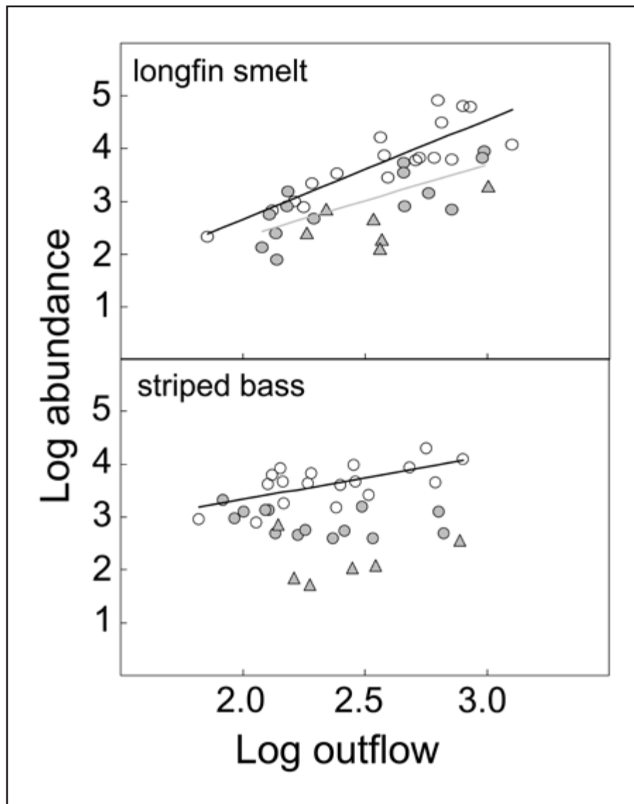
Figure 5. Log-log relationships between fall midwater trawl abundance indices and delta outflow for longfin smelt and young-of-the-year striped bass. Delta outflow values represent the mean levels ( \text{m}^3/\text{s} ) during January–June for longfin smelt, and during April–July for striped bass. The data are compared for pre- Corbula invasion years (1967–1987; white circles), post- Corbula invasion (1988–2000; dark circles), and during the POD years (2001–2006; triangles). Fitted lines indicate linear regression relationships that are statistically significant at the P < 0.05 level.
