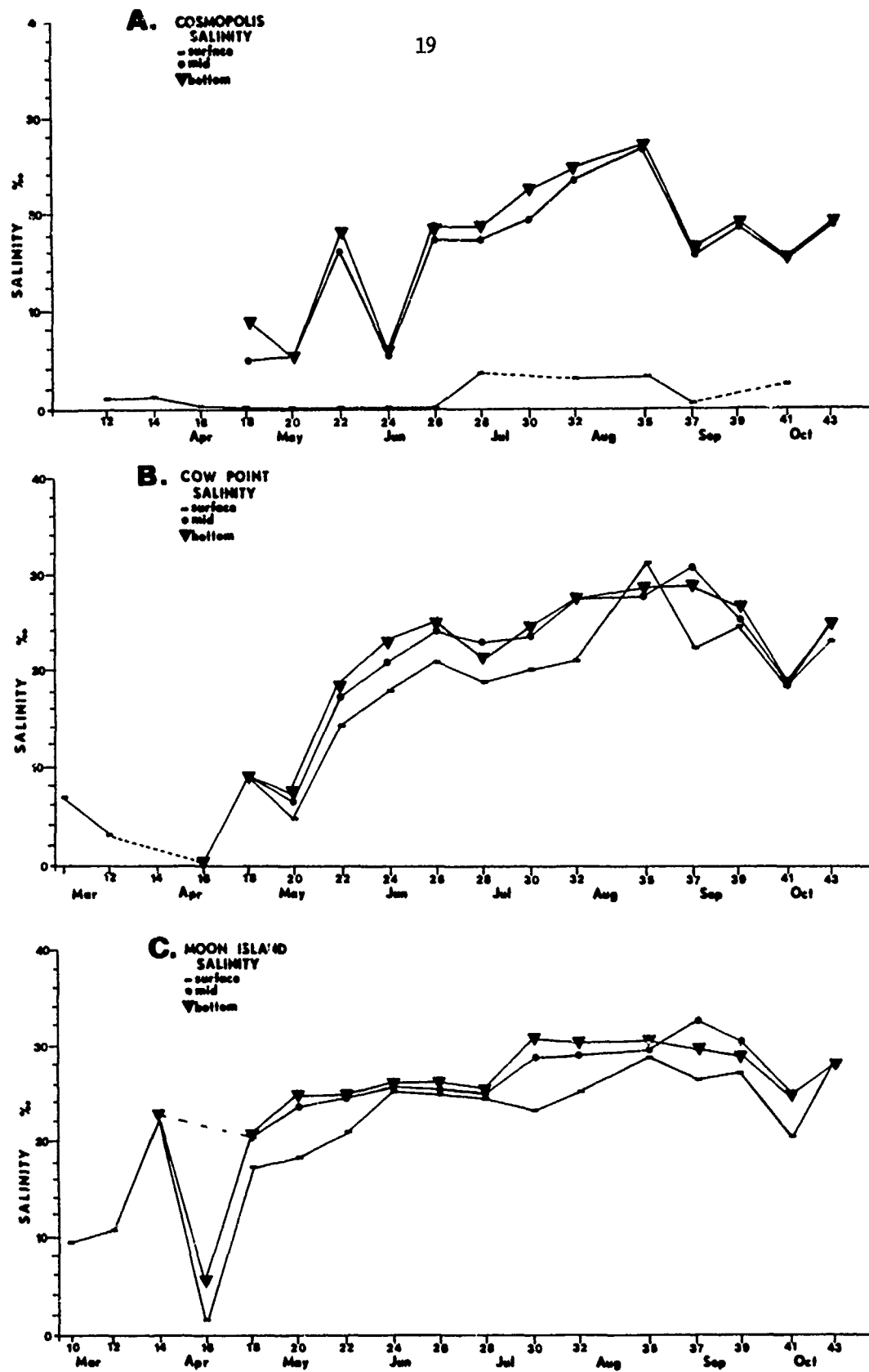
Fig. 2-6. Salinity at three depths at (a) Cosmopolis, (b) Cow Point, (c) Moon Island, (d) Stearn's Bluff, and (e) Westport in Grays Harbor, Washington, March-October 1980.
