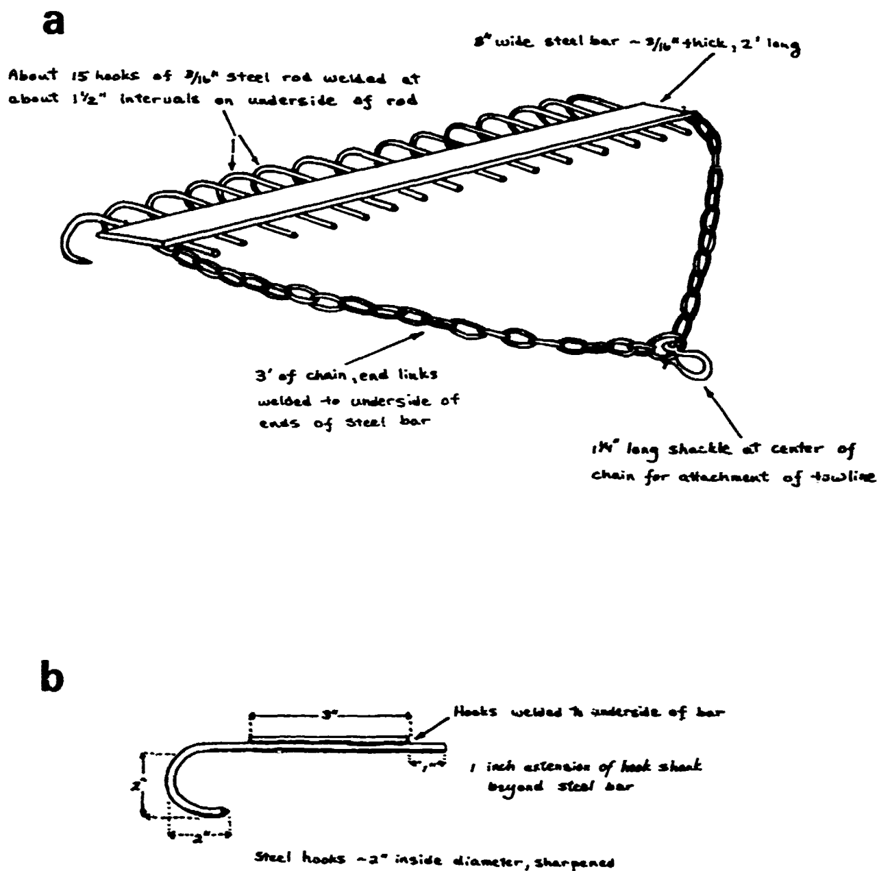
Fig. 5-5. Herring spawn-vegetation sampling rake (a) and detailed view of steel hooks (b) similar to the type utilized to sample for eggs of Pacific herring in Grays Harbor, Washington, March-June 1980. Design and drawing courtesy of Washington Department of Fisheries.
