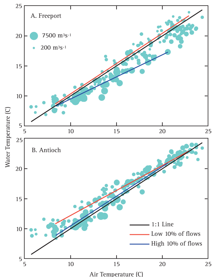
Figure 17. Monthly mean temperature at Freeport and Antioch vs. air temperature at Antioch. Size of symbols indicates freshwater flow. Lines are: Black = 1:1; Red: regression line for the lower 10th percentile of flow; Blue: regression line for upper 10th percentile of flow.
