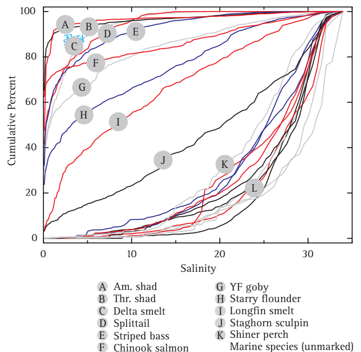
Figure 35. Cumulative salinity distributions of common fish species collected in the IEP San Francisco Bay Study monitoring program. Calculations were as in Figure 33 but the salinity bins were all of equal size. The group of unlabeled lines in the lower right is a suite of marine species including northern anchovy, Pacific herring, white croaker, and jacksmelt.
