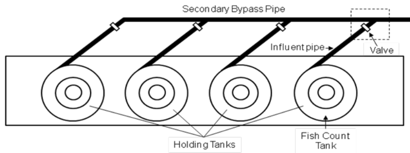
Figure 12. Schematic of the SDFPF's old holding tank building showing location of valve on the holding tank influent pipe.
