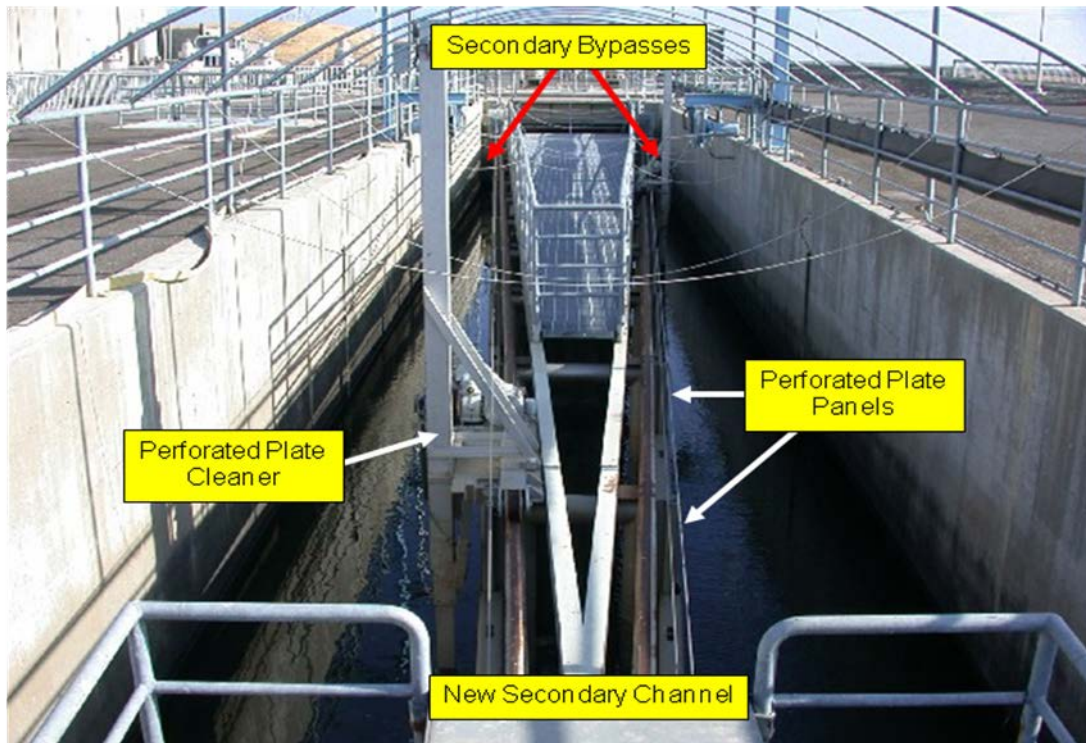
Figure 9. View of the perforated plate system in the new secondary channel.
