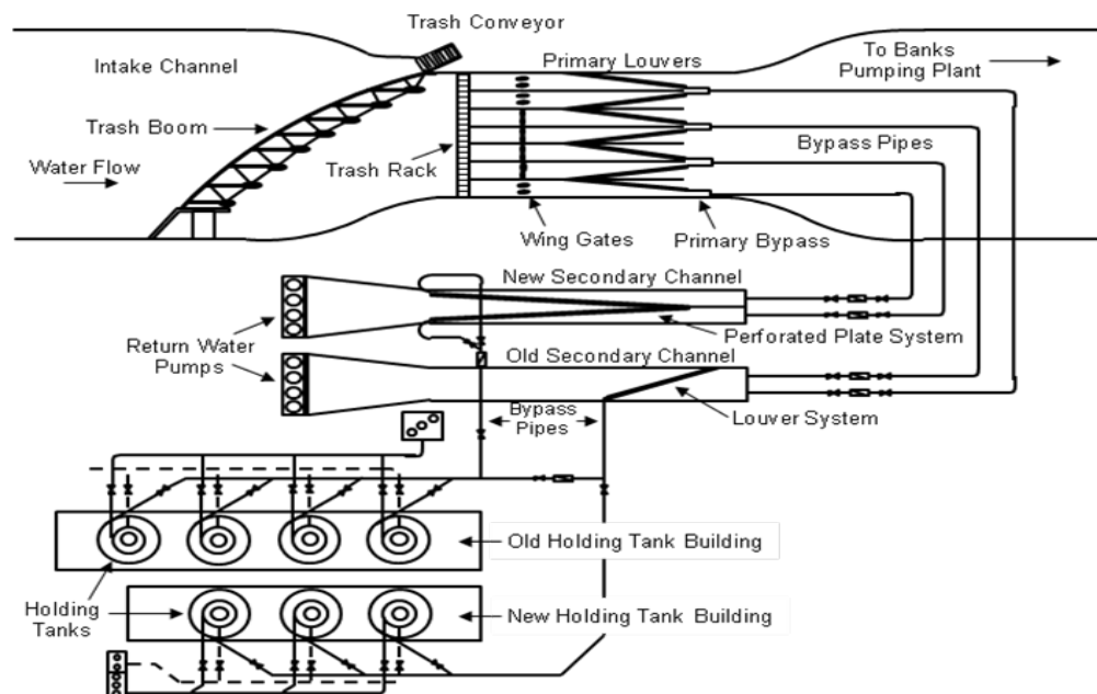
Figure 4. Diagram of the State Water Project's SDFPF.
