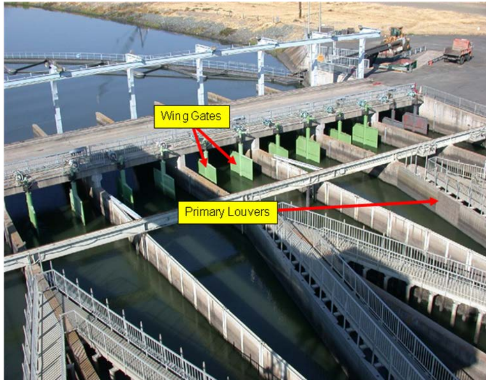
Figure 6. Overhead view of the primary louvers showing the location of the wing gates.
