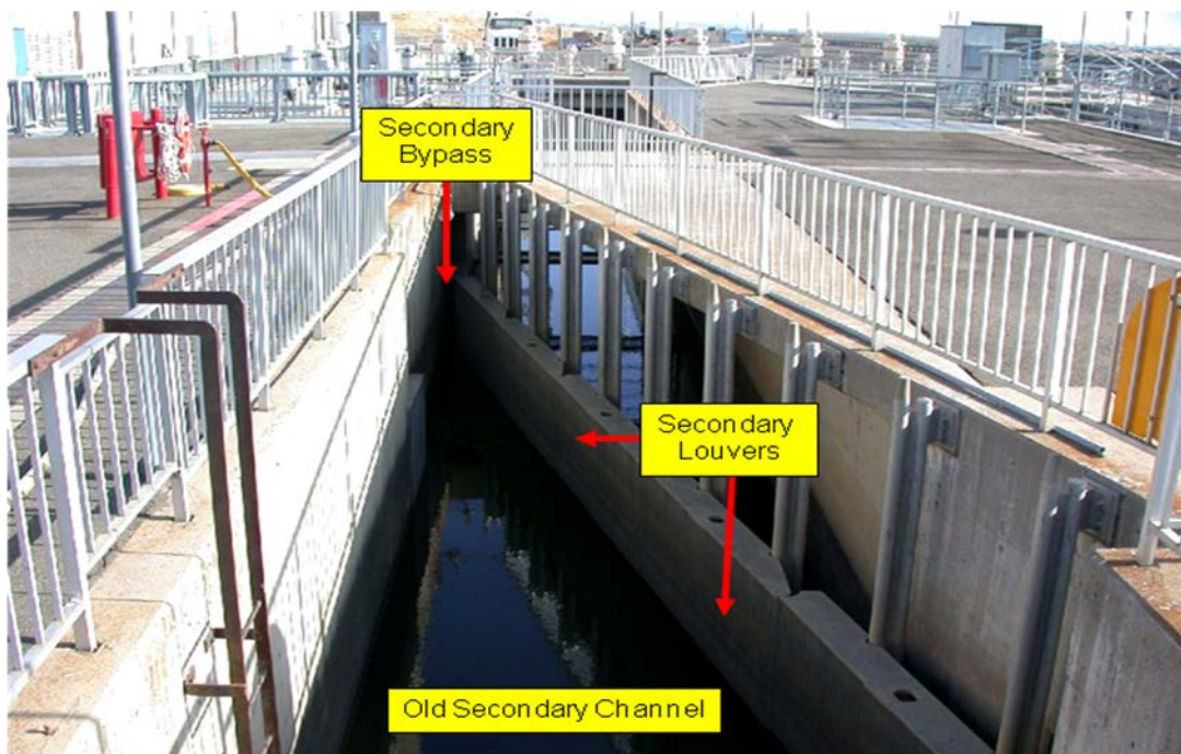
Figure 8. View of the louver system in the old secondary channel.
