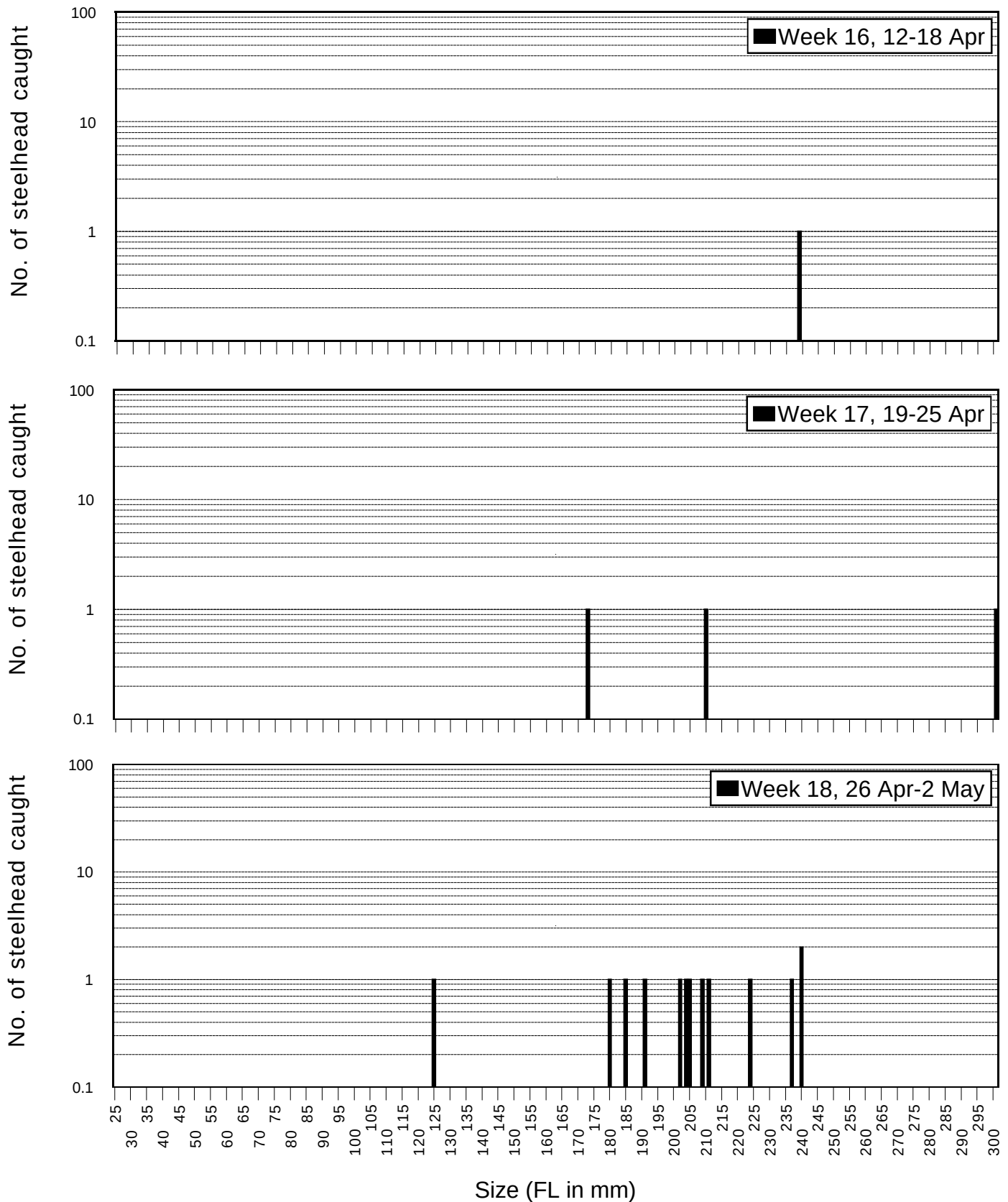
Figure 28. Size distribution of steelhead caught by rotary screw traps at Knights Landing, Sacramento River, 12 April through 02 May 1998.
