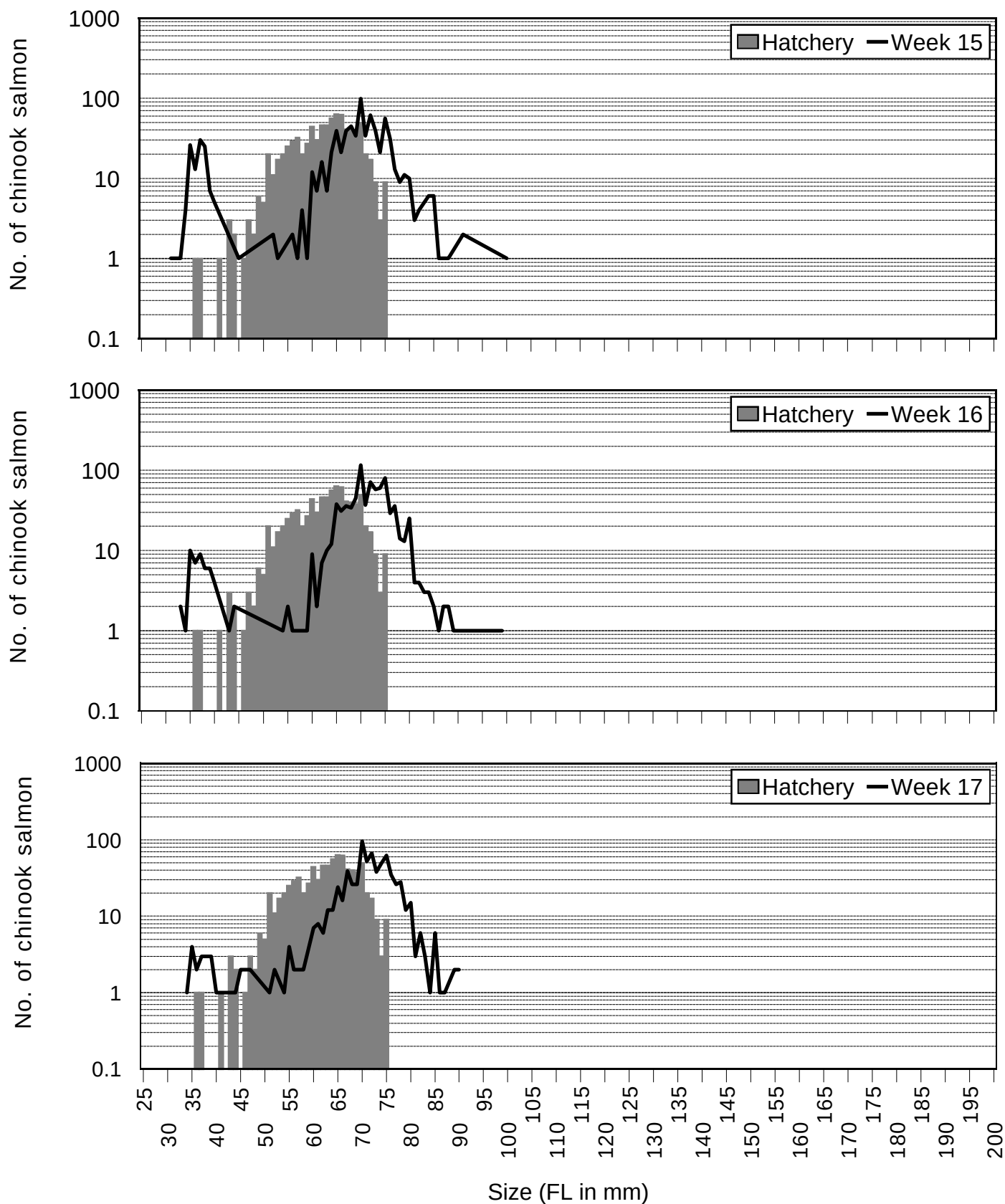
Appendix Figure 4. Size distribution of chinook salmon collected in the Sacramento River near Knights Landing compared with size distribution of Coleman NFH salmon released during week 15 (7 April 1998).
