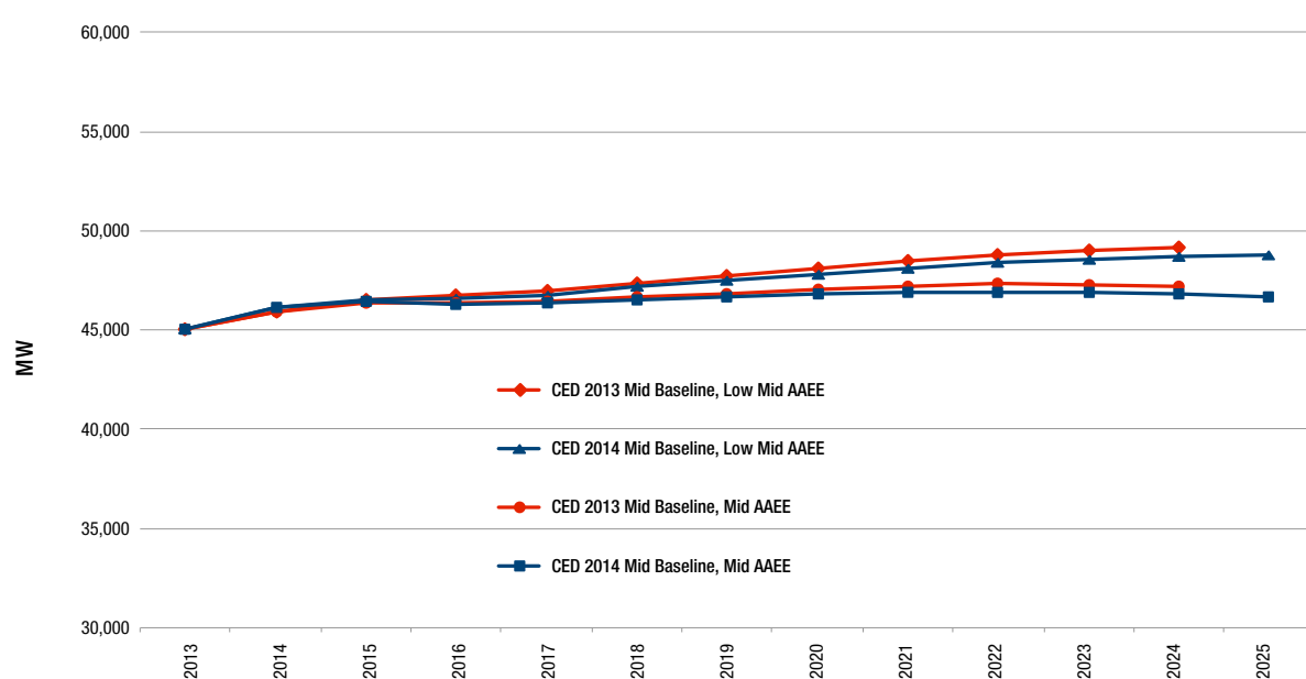
Figure 46: Managed Forecasts for Peak Demand, Combined IOUs
