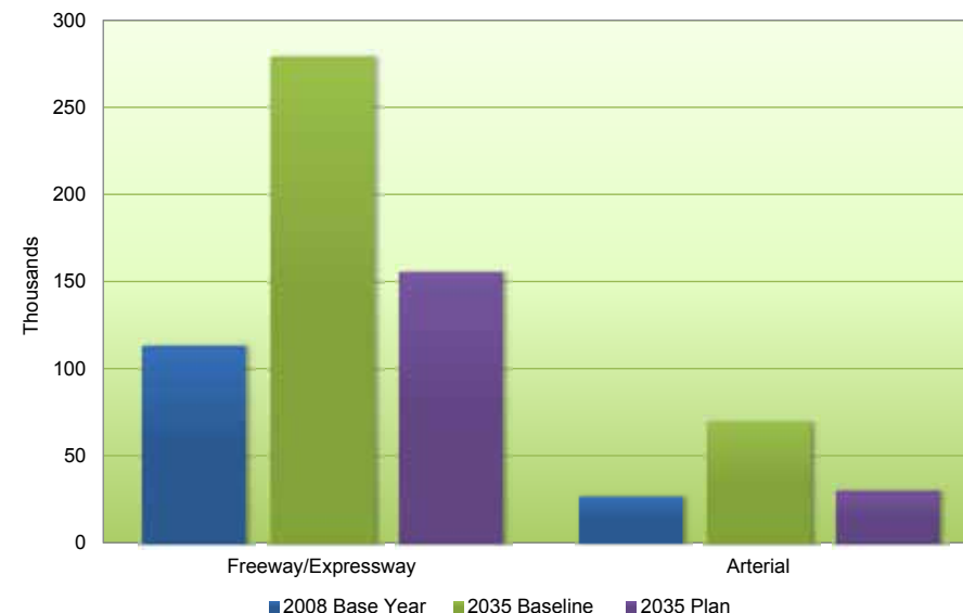
FIGURE 5.3 Daily Heavy-Duty Truck Hours of Delay
