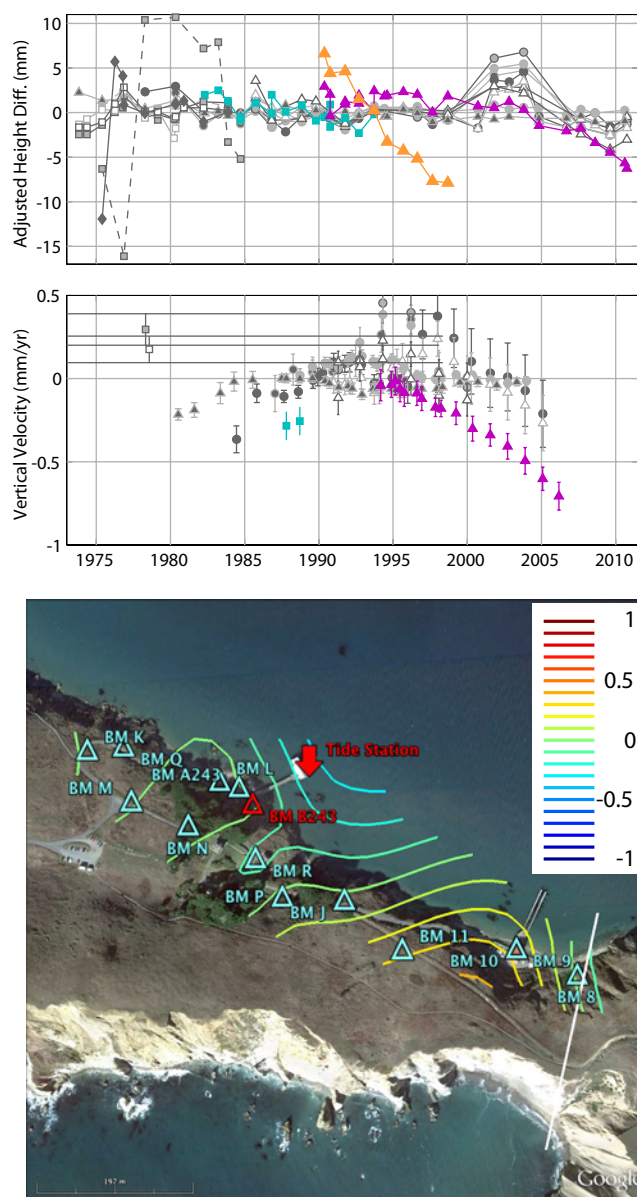
FIGURE D.6 (Top) Time series of vertical displacements for Point Reyes (9415020) tide gage leveling network. All benchmarks shown in gray except tide gage marks AQUAREF (orange), AQUATRAK (magenta) and RM OF ETG (blue). (Middle) Time series of apparent decadal-scale vertical velocities. All benchmarks shown in gray except tide gage marks AQUAREF (orange), AQUATRAK (magenta) and RM OF ETG (blue). (Bottom) Contours of best-fit linear vertical deformation rates for Point Reyes benchmarks with respect to network vertical reference frame. Contours every 0.1 \text{ mm yr}^{-1} . White line indicates mapped fault trace.
