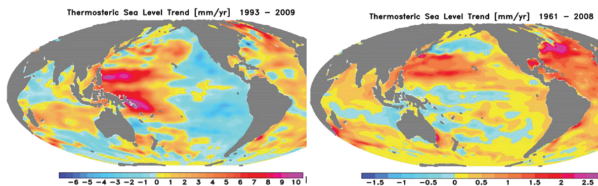
FIGURE 4.1 Trend of thermosteric sea level ( \text{mm yr}^{-1} ) for 1993–2009 ( left ) and 1961–2008 ( right ), based on an updated version of data from Ishii and Kimoto (2009). SOURCE: Courtesy of Masayoshi Ishii, Japan Meteorological Research Institute.
