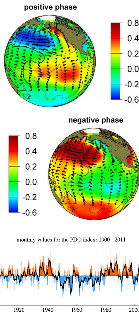
FIGURE The Pacific Decadal Oscillation. (Top) Typical winter patterns of sea surface temperature (colors), sea-level pressure (contours), and surface wind stress (arrows) during positive (warm) and negative (cool) phases of PDO. Temperature anomalies are in degrees Celsius. (Bottom) History of the PDO index (the principal component of monthly sea surface temperature anomalies in the North Pacific Ocean poleward of 20°N) from 1900 to 2010. SOURCE: Figure obtained with permission granted by Nate Mantua at the University of Washington's Joint Institute for the Study of Atmosphere and Ocean.
