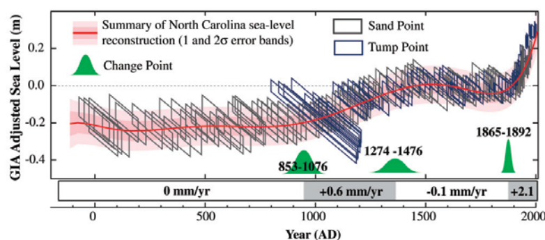
FIGURE Two thousand years of sea-level rise estimates from two North Carolina salt marshes (Sand Point and Tump Point). Errors in the data are represented by parallelograms; the correction for glacial isostatic adjustment is larger at the old end of the error box. The red line is the best fit to the sea-level data. Green shapes indicate when significant changes occurred in the rate of sea-level rise. SOURCE: Kemp et al. (2011).
