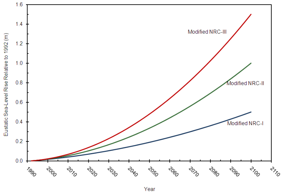
Figure B-11. Scenarios for GMSL Rise (based on updates to NRC 1987 equation).
