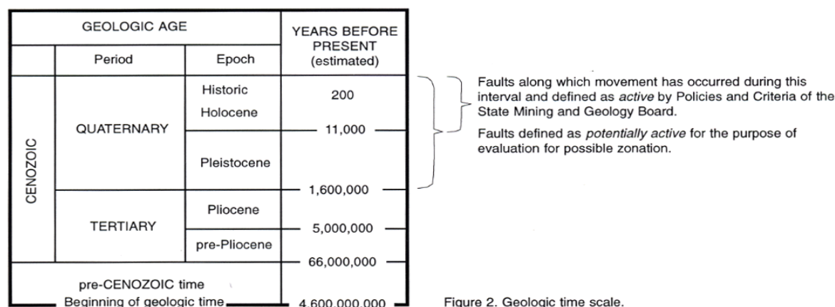
Figure 2. Geologic time scale.
