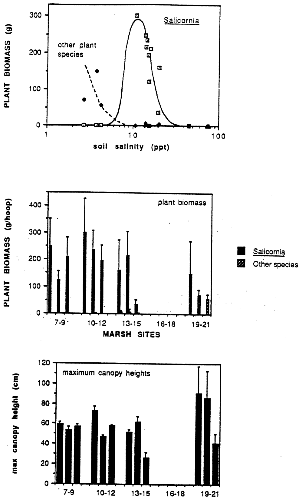
Figure 8. Plant biomass in the marsh sites as a function of soil salinity (A). The mean plant biomass in 1/10m 2 hoops (B) and the maximum canopy heights of the plants in the marsh sites (C); the means of the three seasons ( \pm 1 std. error) are given .
