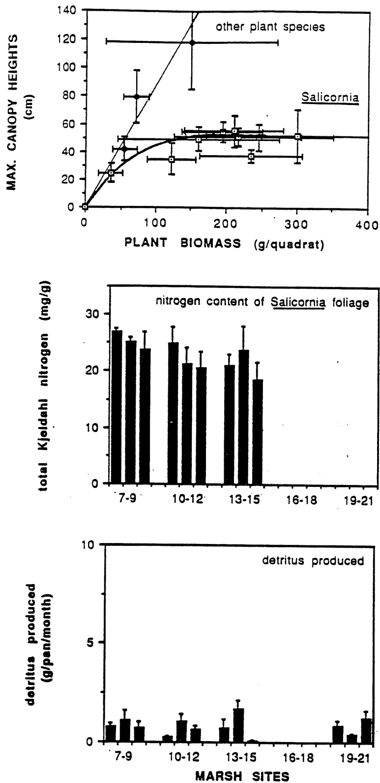
Figure 9. Maximum canopy heights as a function of plant biomass (A); the means of the three samples ( \pm 1 std. deviation) are given for both factors. The nitrogen content of the Salicornia foliage (B) and the detritus produced at the marsh sites. The means of the three seasons ( \pm 1 std. error) are given.
