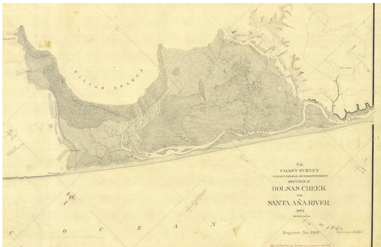
Figure 1. Coastal T-sheet (ca. 1876) showing lateral migration of estuarine mouth.
