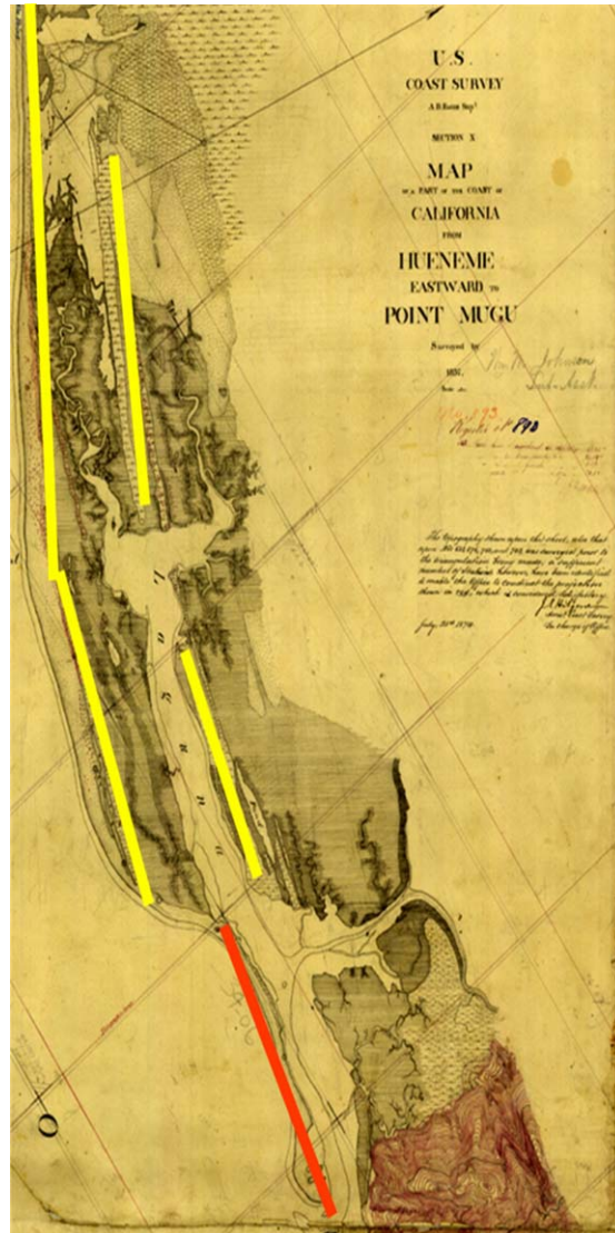
Figure 4. Series of barrier sand spits generating the prograding shoreline and forming much of the space of Mugu Lagoon (ca. 1860).
