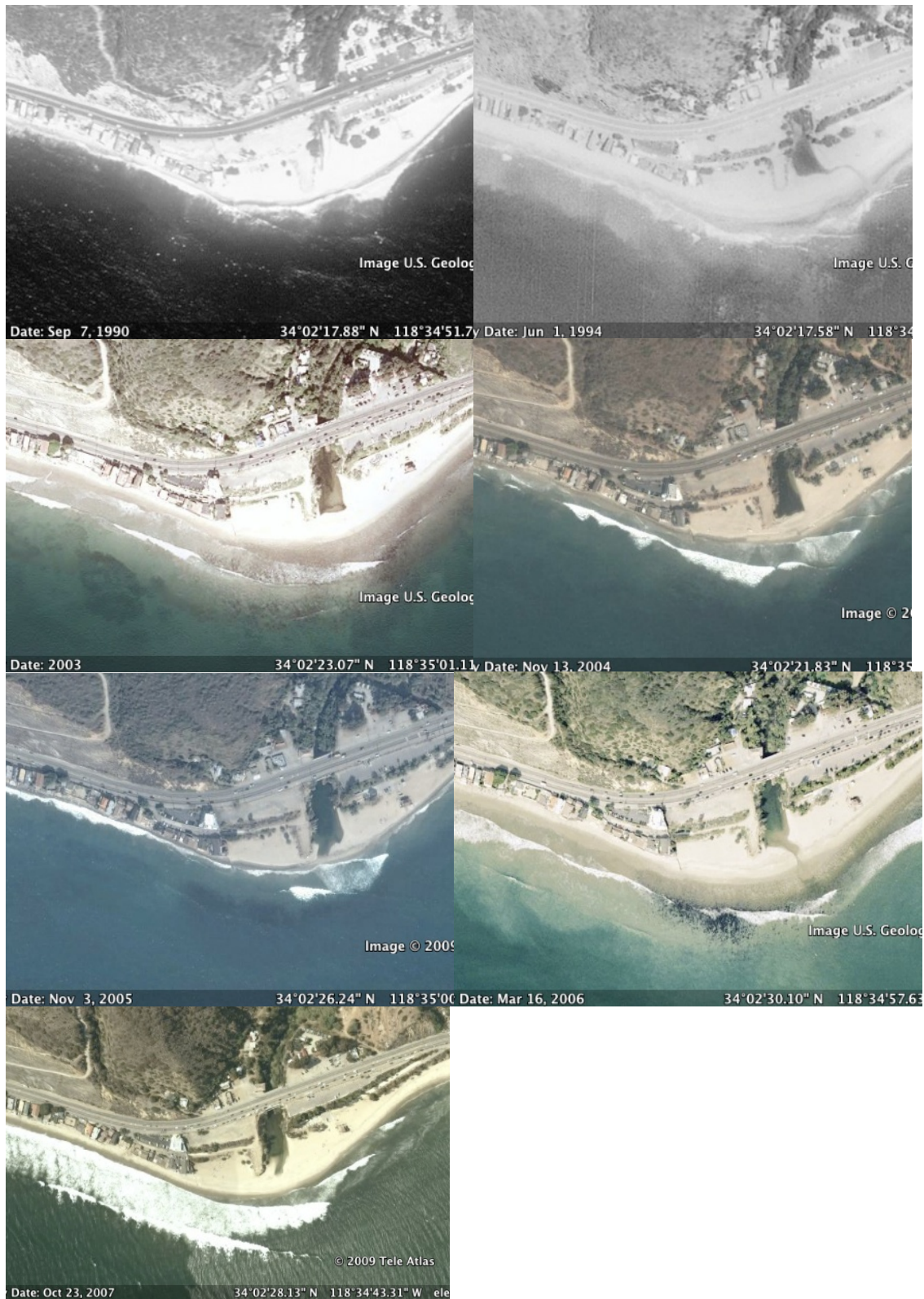
Figure 15. Aerial photographs of Topanga lagoon from Google Earth.
