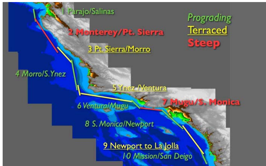
Figure 5. Distribution of coastal settings in southern California. Coastal setting is a regional variable. Here the coast is divided up into 10 units with distinctive properties. Each unit is categorized as to whether it is predominantly prograding, terraced, or steep.
