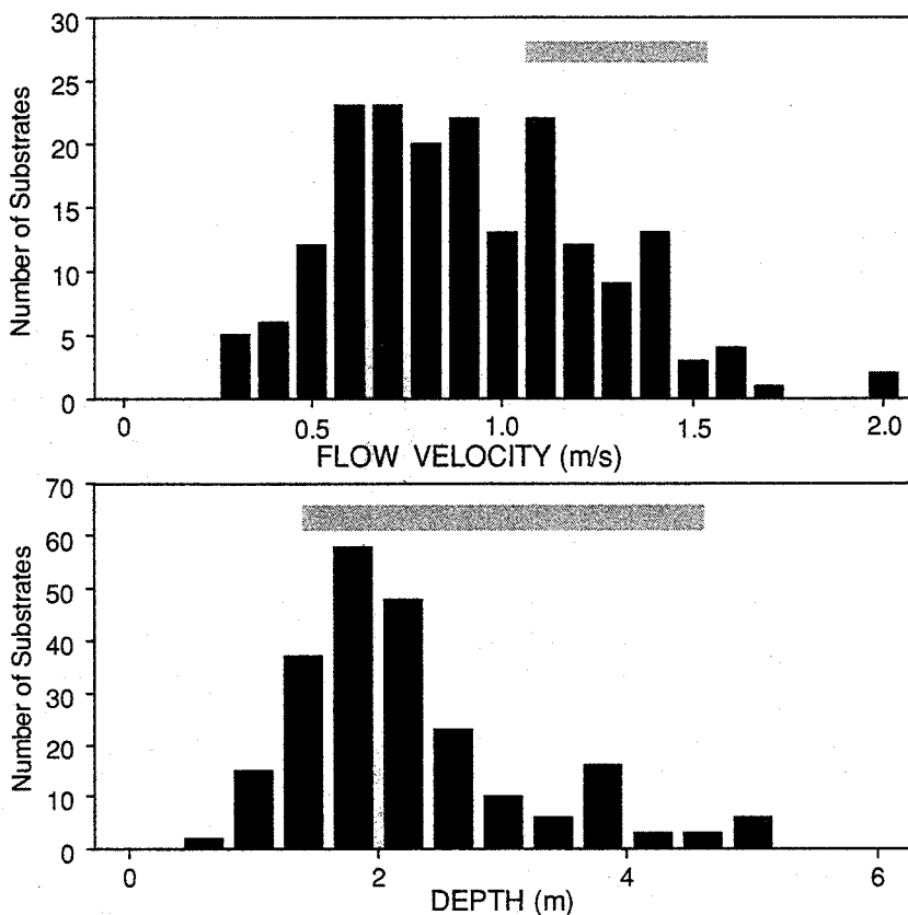
Figure 5. Distribution of bottom flow velocities (measured 30 cm above the substrate) and depths sampled with artificial substrates in the Sacramento River in 1991 and 1992. Shaded horizontal bars denote the range of velocities and depths where eggs were collected.
